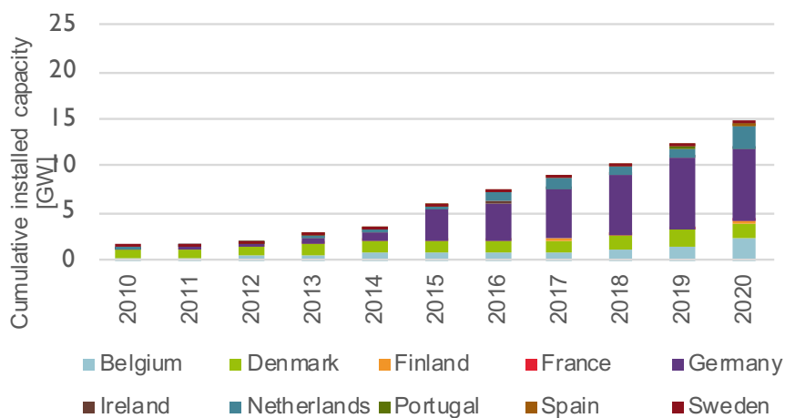
Figure 4.12 EU offshore wind energy installed capacity, MW
